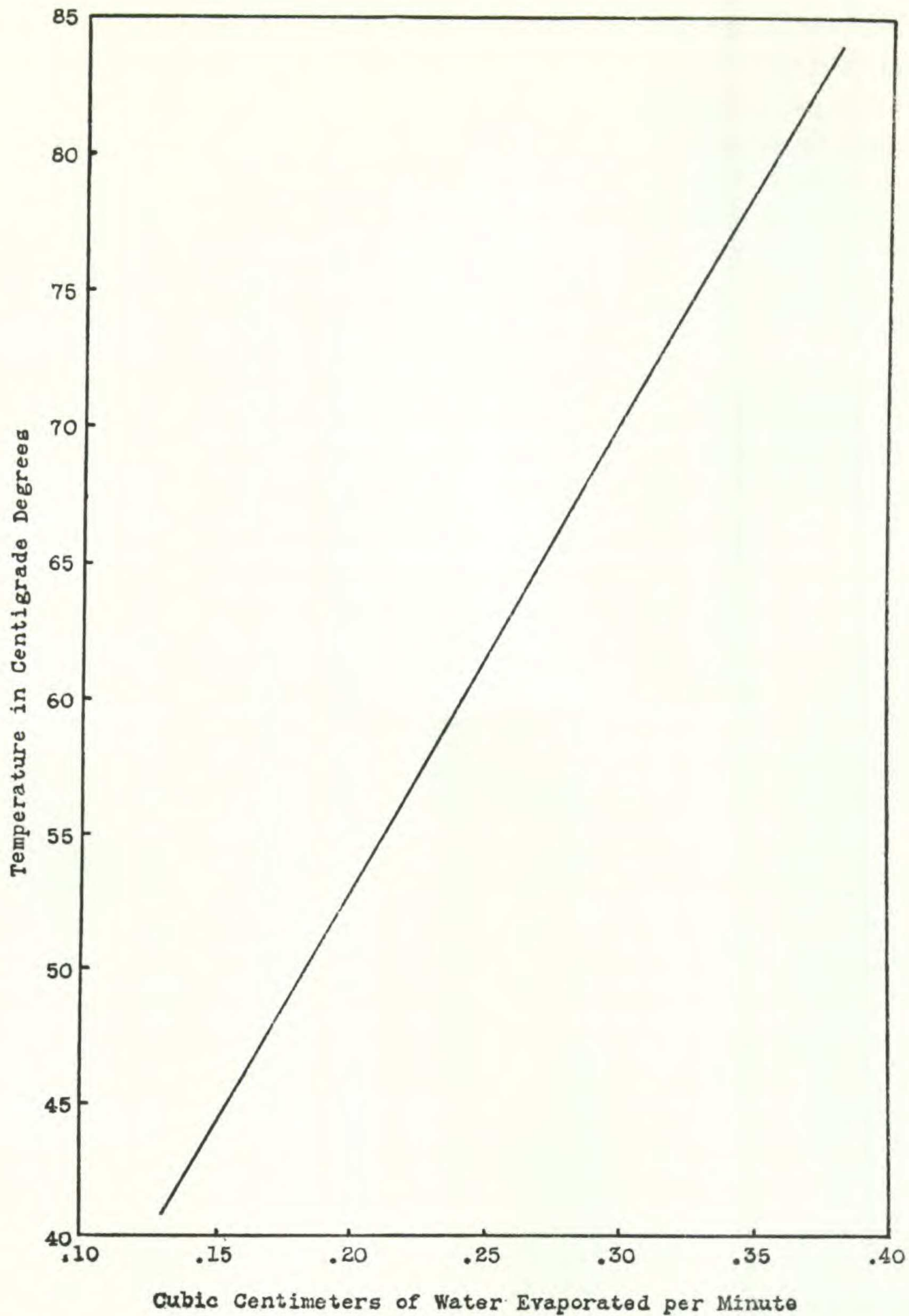
Fig. 2. The number of cubic centimeters of water evaporated per minute from an atometer, plotted against the temperature in Centigrade degrees. The determinations were made at 10^{\circ} intervals. The figures in table II relating to the evaporation rate were taken from this graph.
